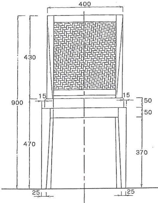
FRONT ELEVATION 1:10
