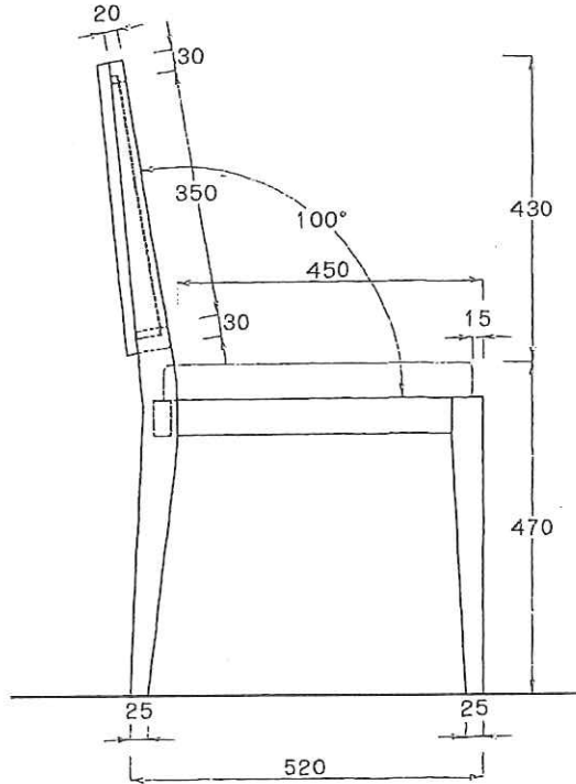
SIDE ELEVATION 1:10
