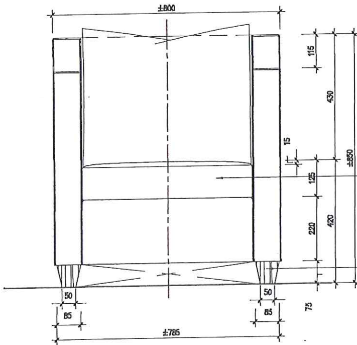
FRONT ELEVATION F-02 LOBBY
