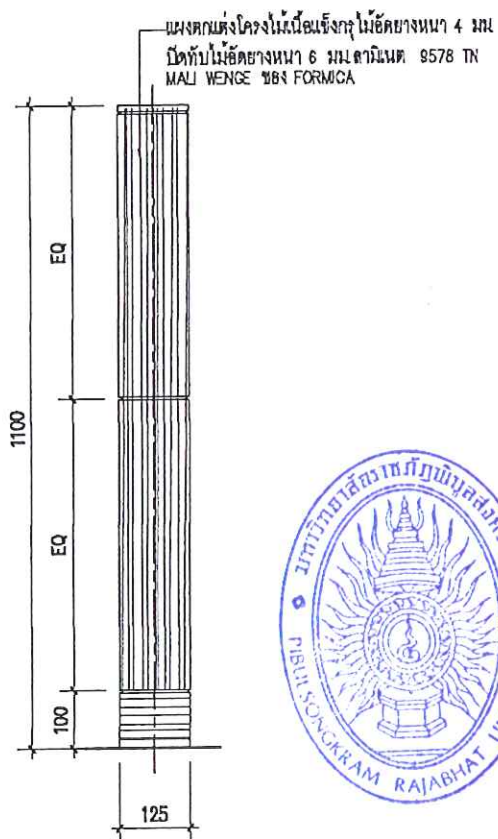
ELEVATION BL-04 LOBBY
