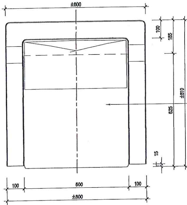
PLAN F-02 LOBBY
