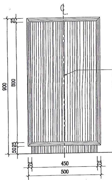
SIDE ELEVATION F-01 LOBBY
